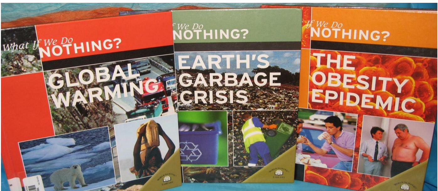
Global Warming
